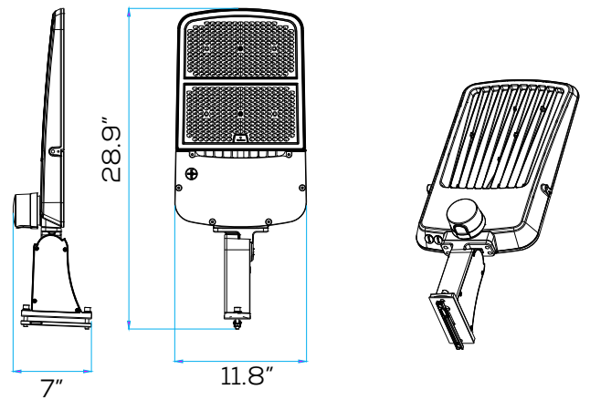
Extruded Mount
