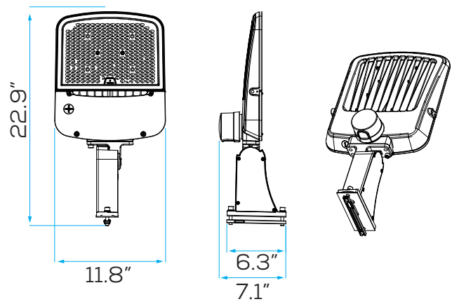
Extruded Arm
