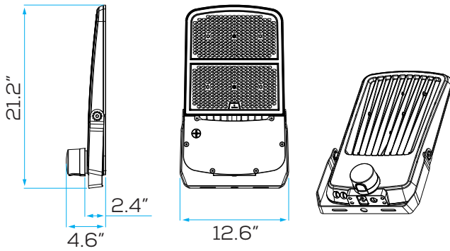
Yoke Mount
